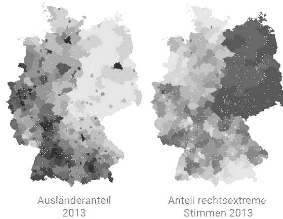
3: Left – Quota of foreigners in the population (darker = higher). Right – Votes in 2013 for right-wing, anti-foreign parties (darker = higher).
